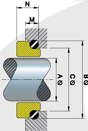
Dimensions (mm)
